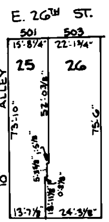
SUB PLAN SCALE 1" = 40'
